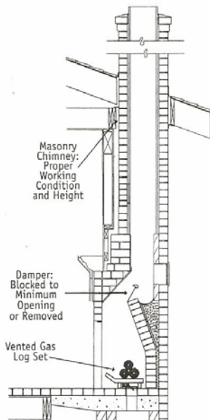
VENTED GAS LOG SET: MASONRY FIREPLACE
