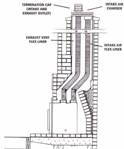
GAS FIREPLACE INSERT: DIRECT VENT INSERT
